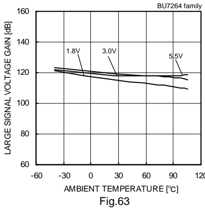
Fig.63 Large Signal Voltage Gain – Ambient Temperature
