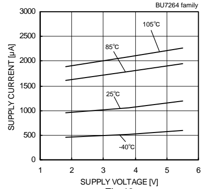
Supply Current – Supply Voltage
