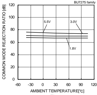
Fig.180 Common Mode Rejection Ratio – Ambient Temperature
