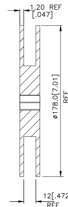
Section C—C
