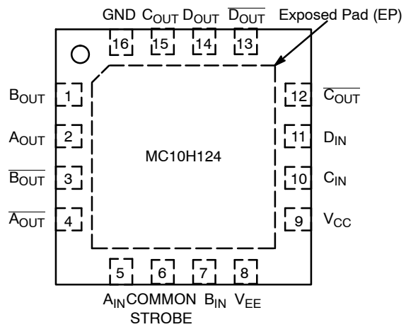
Figure 2. Pin Assignment
