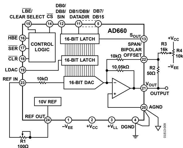
Figure 9. 0 V to 10 V Unipolar Voltage Output with Gain and Offset Adjustment
