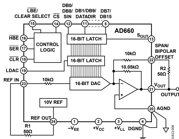
Figure 8. 0 V to 10 V Unipolar Voltage Output
