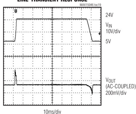
LINE-TRANSIENT RESPONSE
