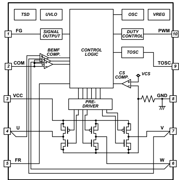
Figure 2. Block Diagram
