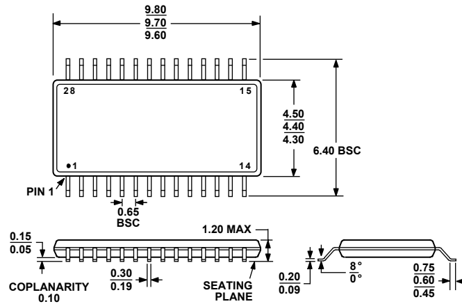
Figure 45. 28-Lead Thin Shrink Small Outline Package [TSSOP]
