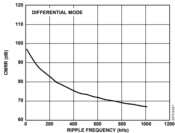
Figure 13. CMRR vs. Common-Mode Ripple with V_{DD} = 5 V and 3 V
