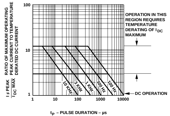
Figure 6. Maximum tolerable peak current vs. pulse duration – Green.
