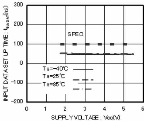
Figure 18. Input Data Setup Time T_{SU:DAT}(\text{HIGH})
