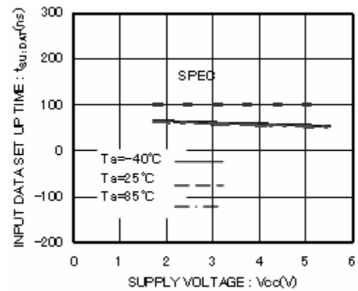
Figure 19. Input Data Setup Time T_{SU:DAT}(\text{LOW})
