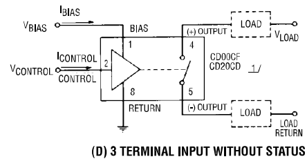
WIRING CONFIGURATIONS FIGURE 1 (SEE NOTE 8)
