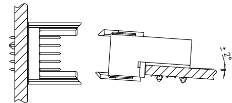
Allowed misalignment
