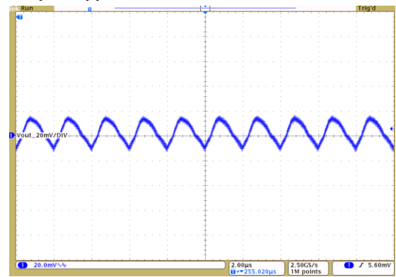
Vout = 20mV/Div, 2.0us/Div Cout = 4 x 100μF Ceramic 331206
