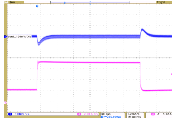
24Vin to 2.5Vout, Cout = 4 x 100μF Ceramic Vout (Ch1) = 100mV/Div, Iout (Ch4) = 2A/Div, 80us/Div 331202
