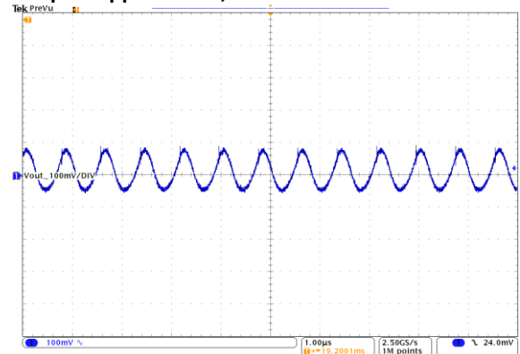
Vout = 100mV/Div, 1us/Div Cout = 4x22μF Ceramic 330506
