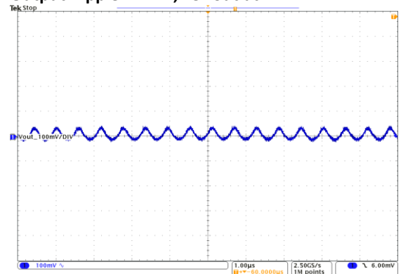
Vout = 100mV/Div, 1us/Div Cout = 4x22μF Ceramic 330507
