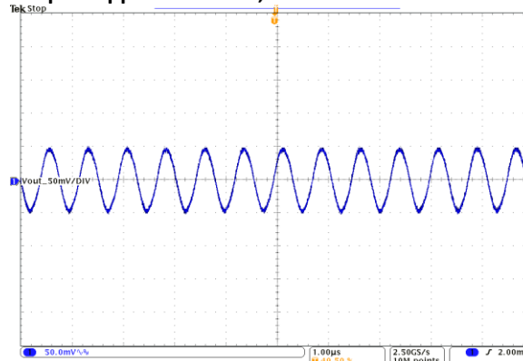
Vout = 50mV/Div, 1.0us/Div
