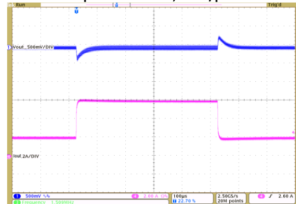
24Vin to 15.0Vout Cout = 4x22μF Ceramic 330504
