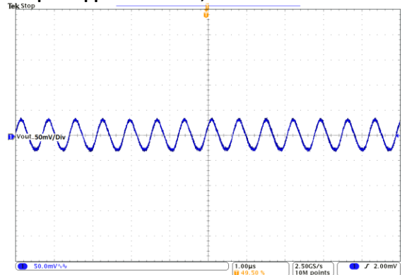
Vout = 50mV/Div, 1.0us/Div
