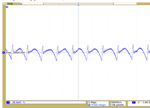
Output Ripple: 24Vin, 1.8Vout at 10A
