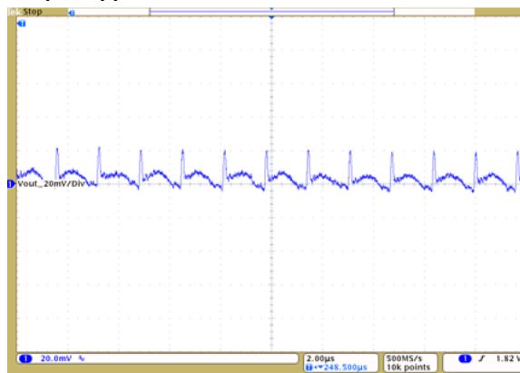
Output ripple: 24Vin, 1.8Vout at 5A
