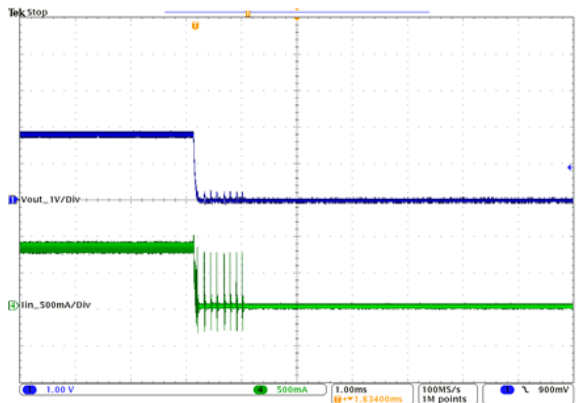
Short Circuit Test
