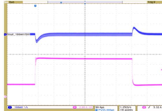
24Vin to 2.5Vout, Cout = 4 x 100μF Ceramic Vout (Ch1) = 100mV/Div, Iout (Ch4) = 2A/Div, 80us/Div
