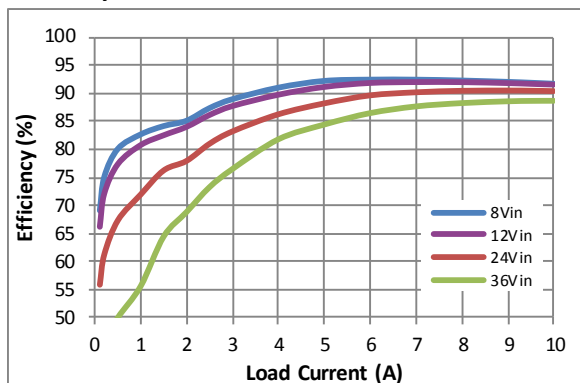
Efficiency at 25°C
