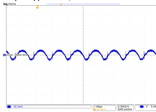
Vout = 50mV/Div, 1.0us/Div
