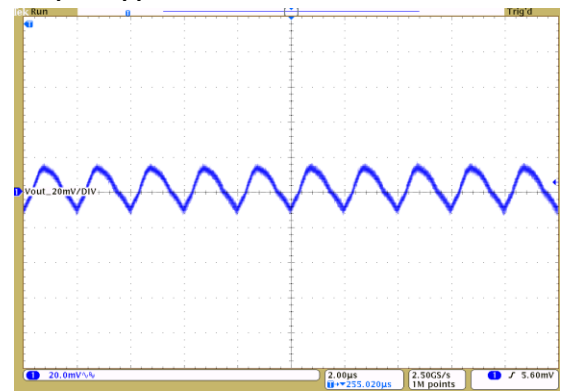
Vout = 20mV/Div, 2.0us/Div Cout = 4 x 100μF Ceramic
