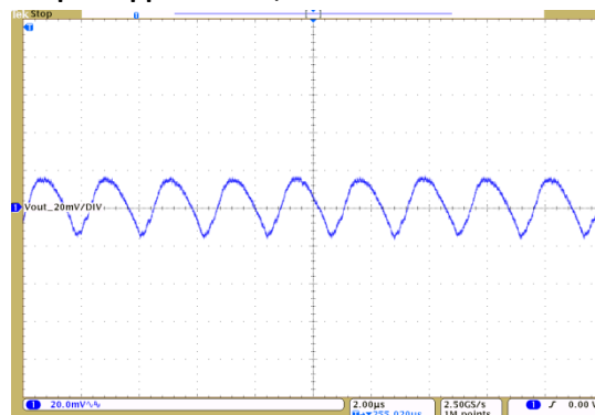
Vout = 20mV/Div, 2.0us/Div
