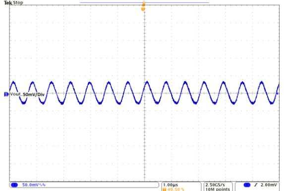
Vout = 50mV/Div, 1.0us/Div Cout = 4 X 22uF Ceramic
