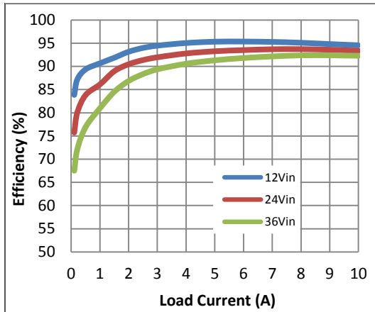
Regulator and inductor performance
