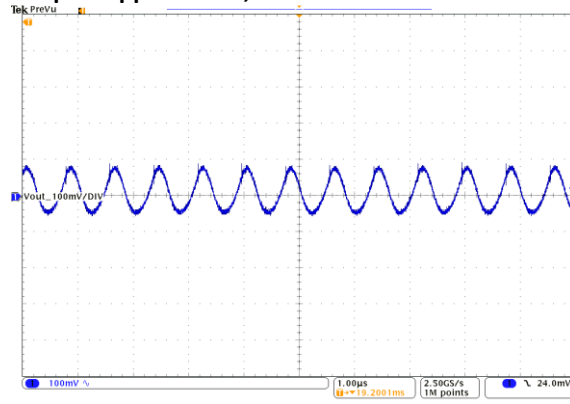
Vout = 100mV/Div, 1us/Div Cout = 4x22μF Ceramic 330506
