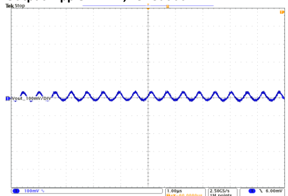
Vout = 100mV/Div, 1us/Div Cout = 4x22μF Ceramic 330507
