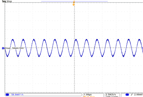
Vout = 50mV/Div, 1.0us/Div Cout = 4 X 22uF Ceramic
