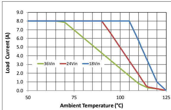
Load Current vs. Ambient Temperature, 0 LFM
