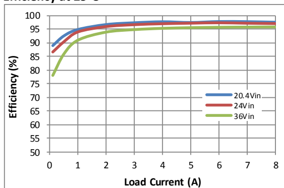
Regulator and inductor performance 330501
