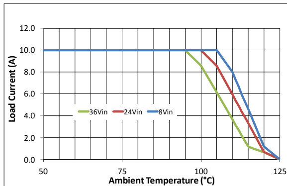
Load Current vs. Ambient Temperature, 400 LFM
