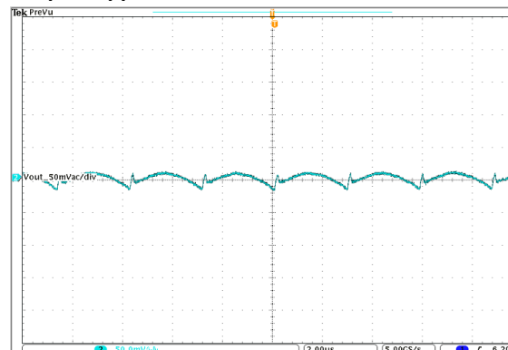
Vout = 50mV/Div, 2.0us/Div
