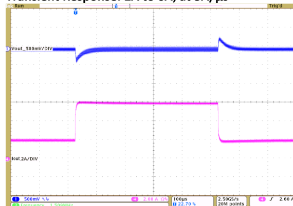
24Vin to 15.0Vout Cout = 4x22μF Ceramic 330504
