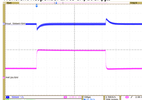
24Vin to 15.0Vout
