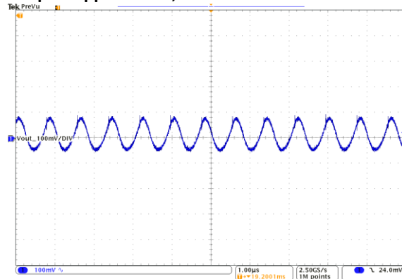
Vout = 100mV/Div, 1us/Div
