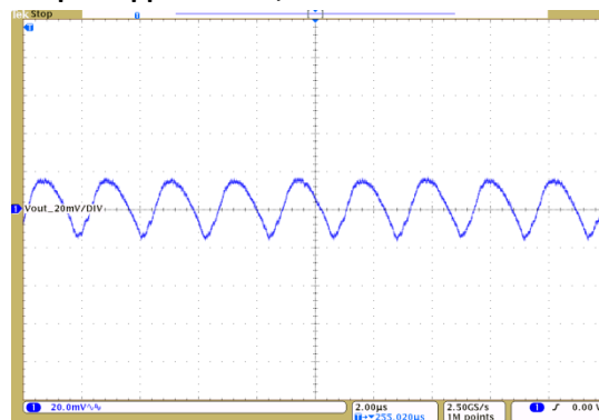
Vout = 20mV/Div, 2.0us/Div Cout = 4 x 100μF Ceramic 331204
