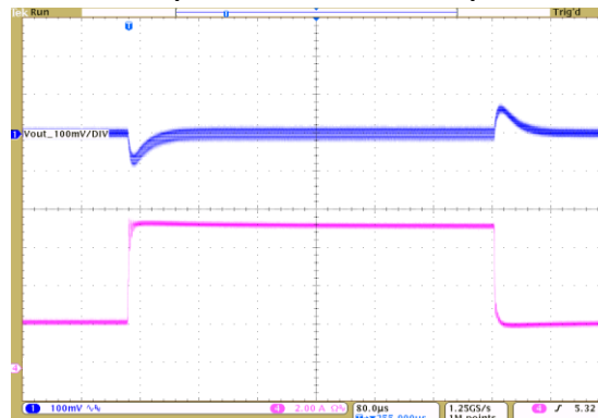
24Vin to 2.5Vout, Cout = 4 x 100μF Ceramic Vout (Ch1) = 100mV/Div, Iout (Ch4) = 2A/Div, 80us/Div 331202
