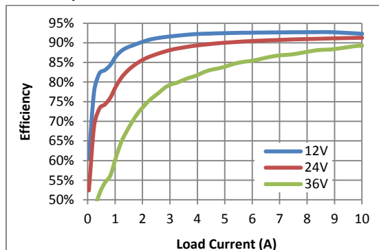
Regulator and inductor performance 331201
