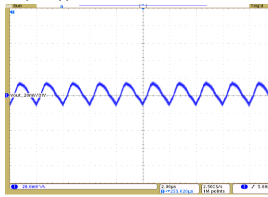
Vout = 20mV/Div, 2.0us/Div Cout = 4 x 100μF Ceramic 331206
