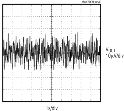
0.1Hz TO 10Hz OUTPUT NOISE ( V_{OUT} = 2.048V )
