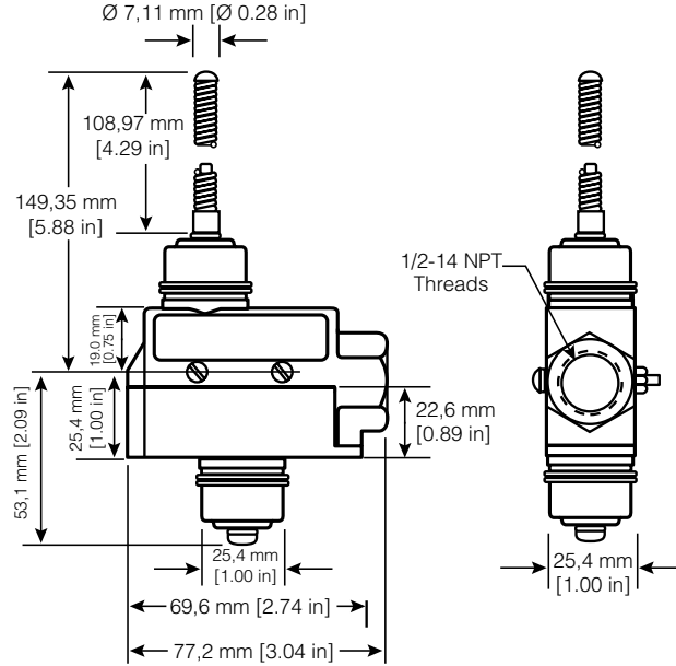
Figure 13. Coil wobble plunger, reset, side mount with boot seal
