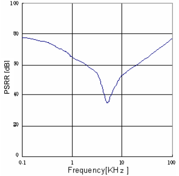
Fig.32 PSRR ( I_o=0mA )
