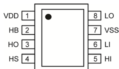
MIC4604YM 8-Pin SOIC (M) (Top View)
