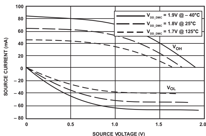
Figure 57. Driver Type C Current (1.8 V V_{DD\_DMC} )
