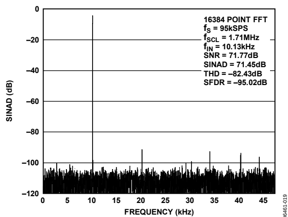
Figure 16. Dynamic Performance, f_{\text{SCL}} = 1.71\text{ MHz} Without Clock Stretching, V_{\text{DD}} = 5\text{ V} , Full-Scale Input, Seven-Term Blackman-Harris Window
