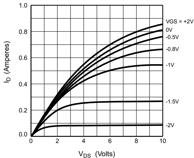
Saturation Characteristics
