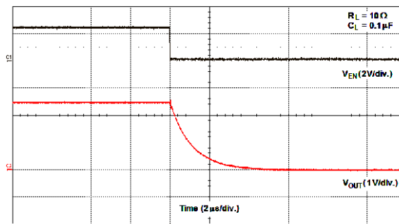
Figure 27 - SiP32451 and SiP32452 Turn-Off Time ( V_{IN} = 2.5\text{ V} )
