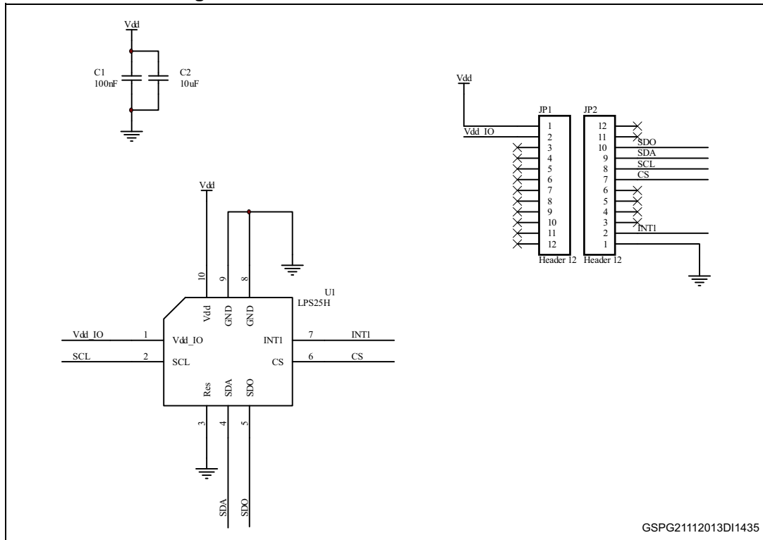
Figure 1. STEVAL- MKI142V1 circuit schematic
