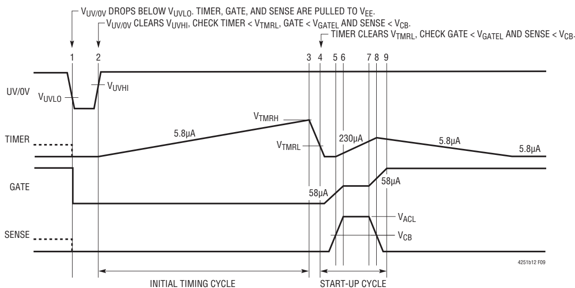
Figure 9. Undervoltage Lockout Timing (All Waveforms are Referenced to V_{FF} )
