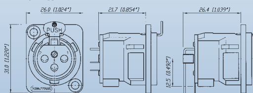
NC3MD-V / NC3MD-H
