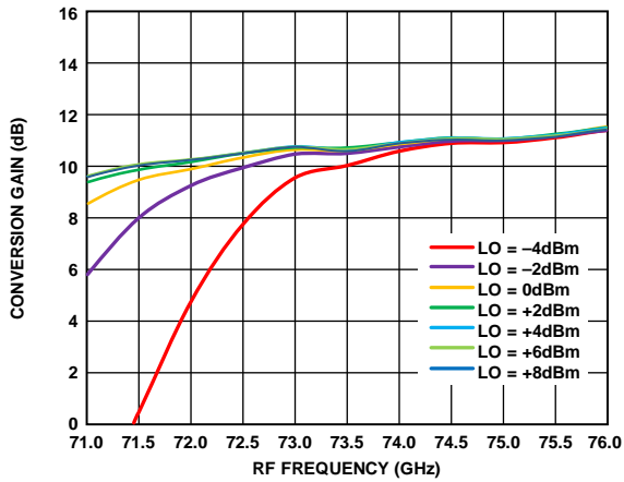
Figure 141. Conversion Gain vs. RF Frequency at Various LO Powers, RFIN = -20 dBm, IF = 1000 MHz, VDLNA = 4 V
