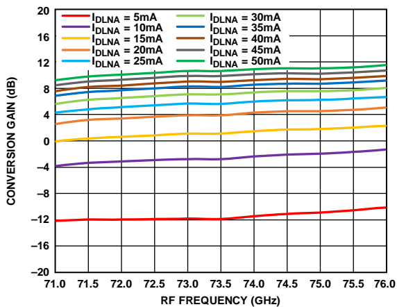
Figure 142. Conversion Gain vs. RF Frequency at Various IDLNA Values, RFIN = -20 dBm, IF = 1000 MHz, VDLNA = 4 V
