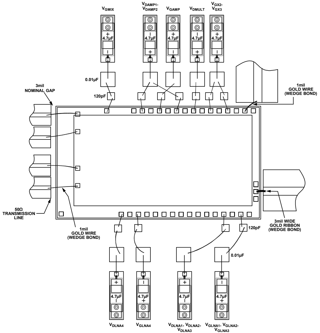
Figure 213. Assembly Diagram
