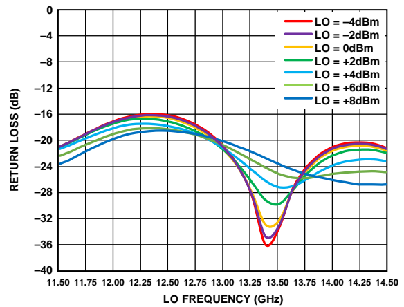
Figure 43. LO Return Loss vs. LO Frequency at Various LO Powers, V DLNA = 4 V
