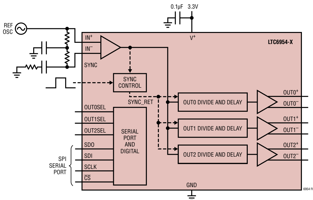
Figure 7. SYNC_RET Propagation
