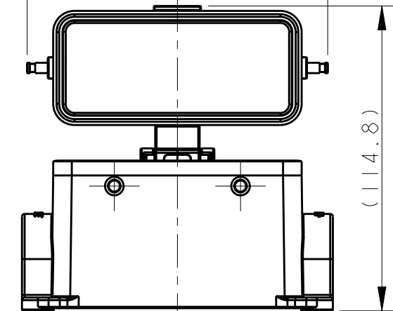
TYPE 2: BODY + 4 EAR + METAL PROTECTION COVER
