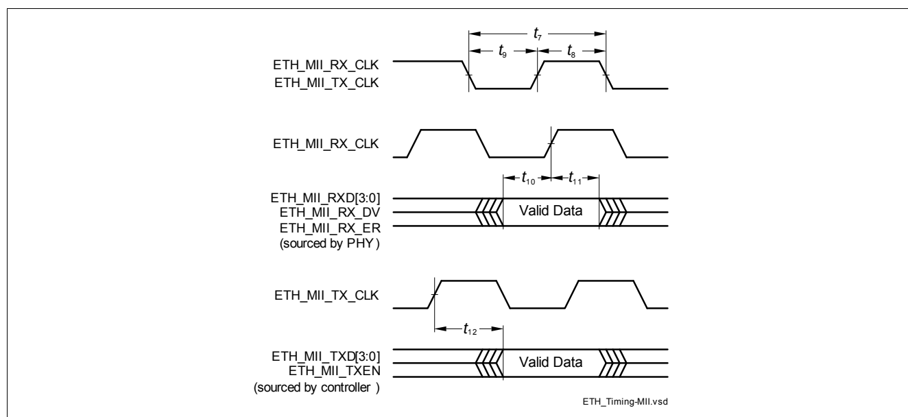
Figure 3-17 ETH MII Signal Timing
