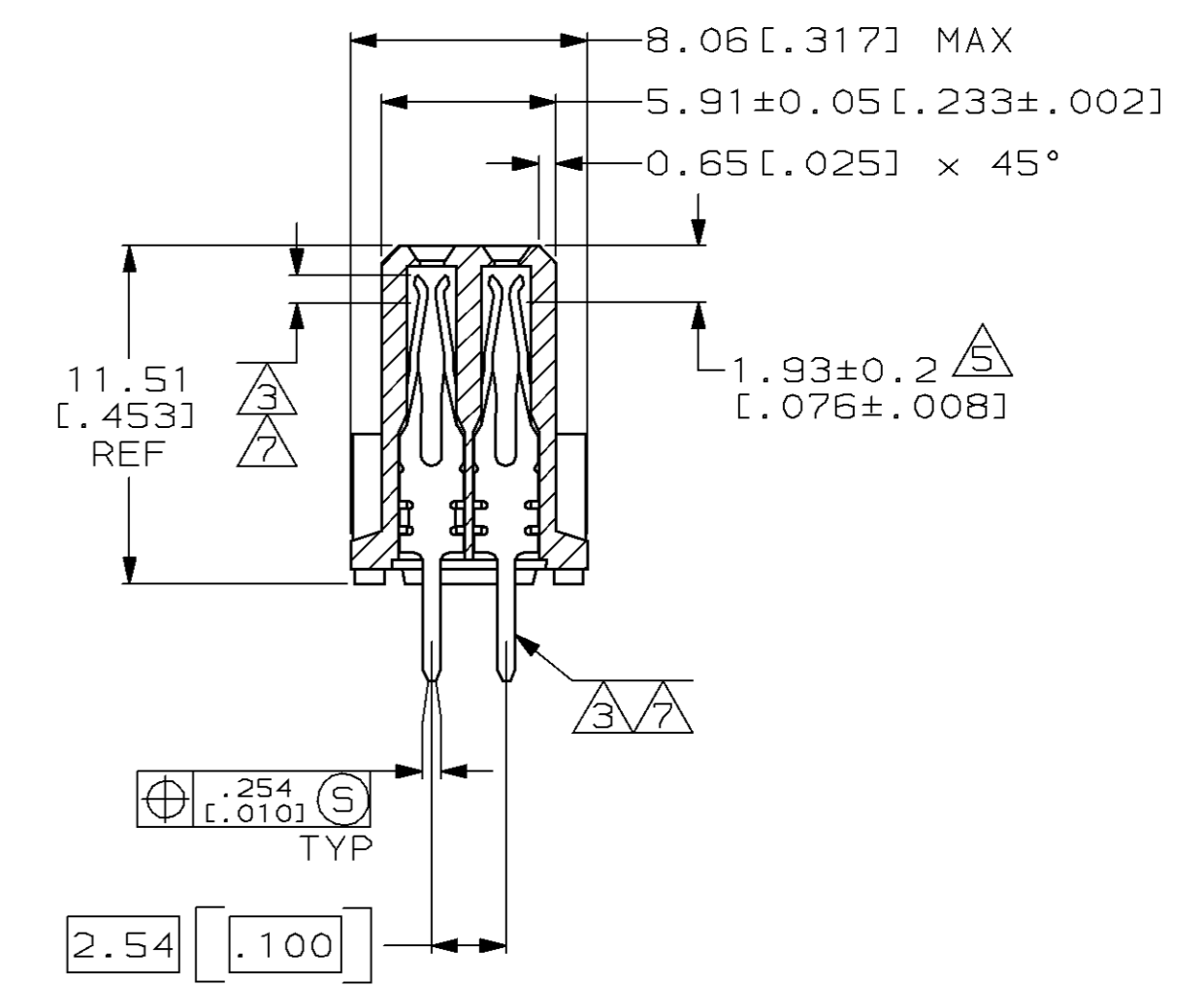
SECTION X-X
