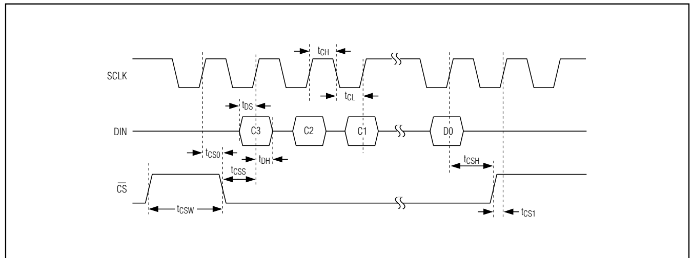
Figure 1. Timing Diagram
