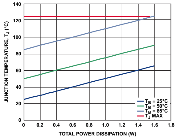
Figure 61. Junction Temperature vs. Total Power Dissipation and Board Temperature
