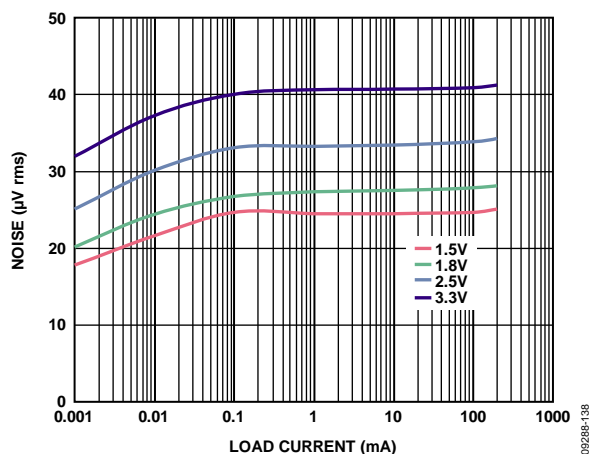
Figure 40. 100 Hz to 100 kHz Output Noise vs. Load Current and Output Voltage, V_{IN} = 5 V , V_{RIPPLE} = 50 mV , C_{OUT} = 1 \mu F
