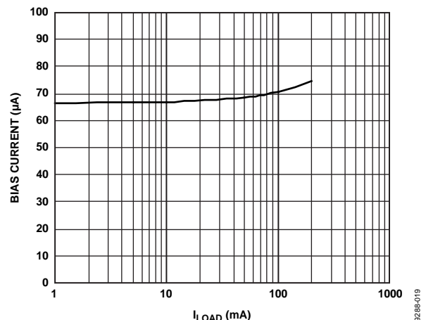
Figure 21. Bias Current vs. Load Current, Single Output Loaded, V_{RIPPLE} = 50\text{ mV} , C_{OUT} = 1\text{ }\mu\text{F}
