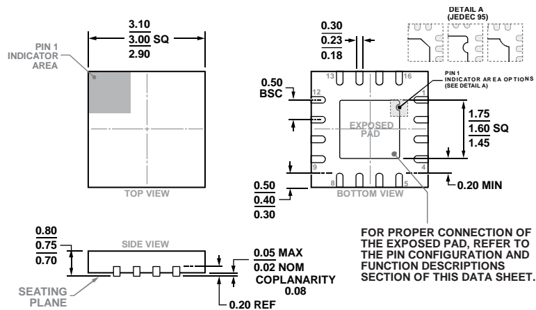
Figure 64. 16-Lead Lead Frame Chip Scale Package [LFCS] 3 mm × 3 mm Body and 0.75 mm Package Height (CP-16-22) Dimensions shown in millimeters
