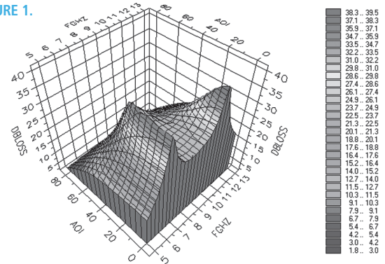
VBROP can optimize absorber performance at various frequencies and angles of incidence.
