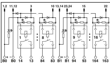
Output base module with 16 miniature relays, 1 N/O contact
