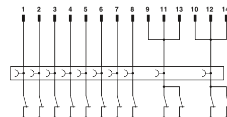
FLKM 14/KDS3-MT/PPA/PLC connection scheme
