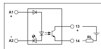
Figure 3: 2-wire output
