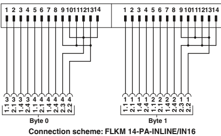
Connection scheme: FLKM 14-PA-INLINE/IN16
