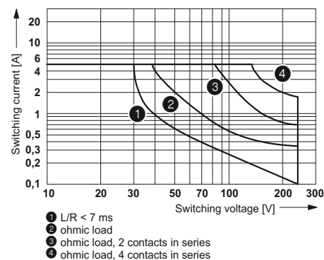
DC interrupting rating
