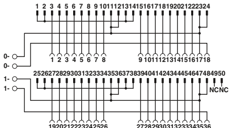
Connection scheme: FLKM 50-PA-AB/1756/IN/EXTC
