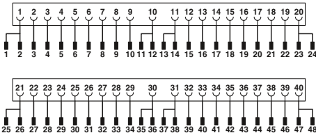
Connection scheme FLKM 50-PA-S300/SO167
