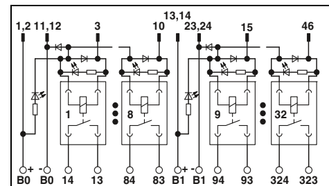
Output module with 32 miniature relays, 1 N/O contact
