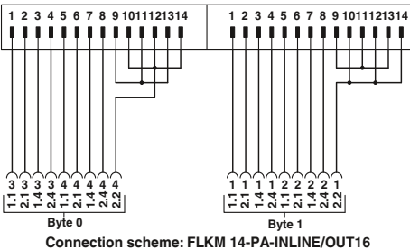
Connection scheme: FLKM 14-PA-INLINE/OUT16
