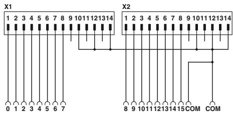
Connection scheme FLKM 14-PA-SLC500/IN
