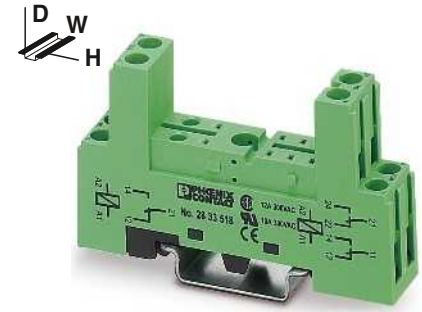
2/2-level design with screw connection
