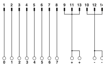
VIP-2/SC/FLK14/PLC connection scheme
