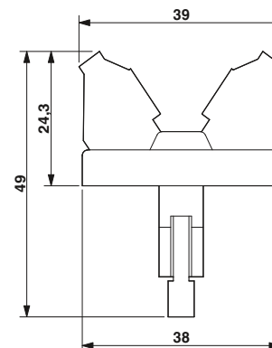
Dimensional drawing DFLK:
