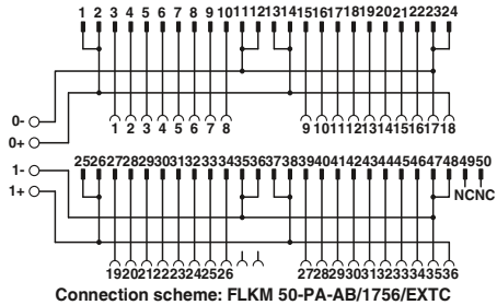
Connection scheme: FLKM 50-PA-AB/1756/EXTC
