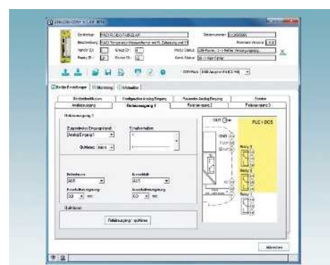
Relay configuration
