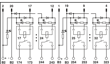
Output extension module with 16 miniature relays, 1 N/O contact
