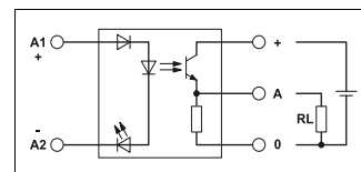
Figure 4: 3-wire output
