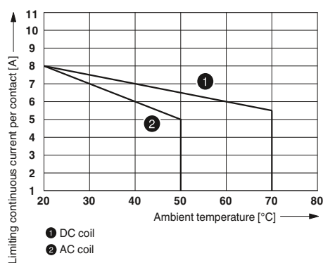
Contact derating
