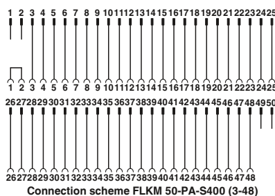
Connection scheme FLKM 50-PA-S400 (3-48)
