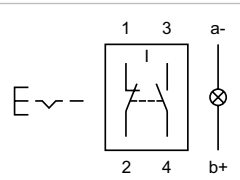
Wiring diagram 25
