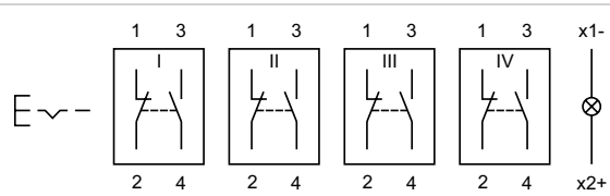
Wiring diagram 23
