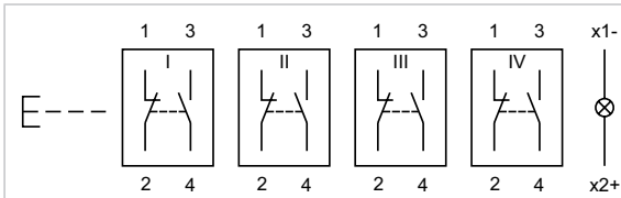
Wiring diagram 22
