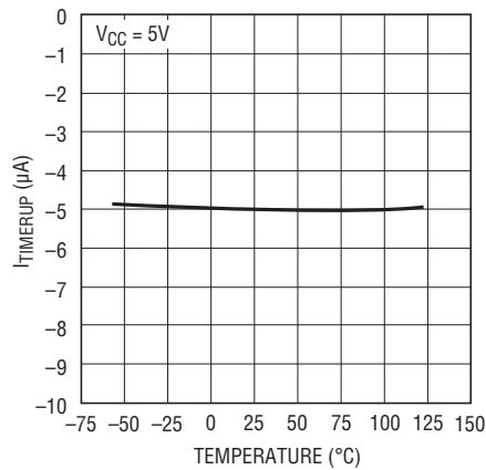
I_{\text{TIMERUP}} (In Initial Cycle) vs Temperature
