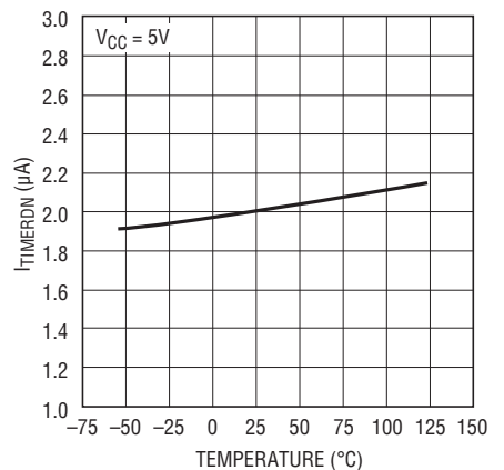
I_{\text{TIMERDN}} (In Cool-Off Cycle) vs Temperature
