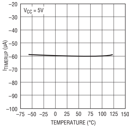
I_{\text{TIMERUP}} (During Circuit Breaker Delay) vs Temperature
