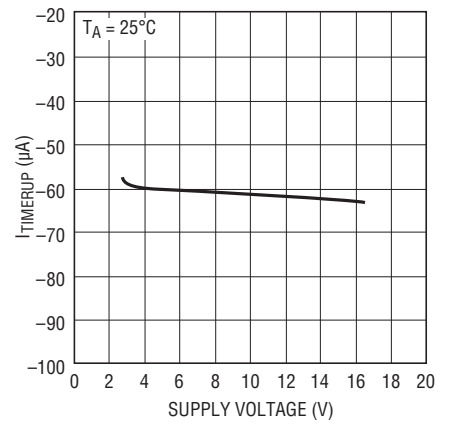
I_{\text{TIMERUP}} (During Circuit Breaker Delay) vs Supply Voltage
