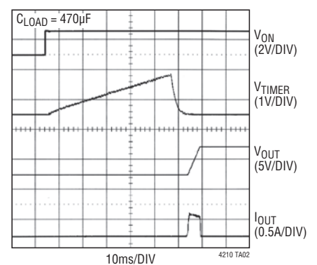
Power-Up Sequence
