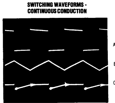
A = Switch Voltage (LX) 5V/div (4.8V to -5.3V) B = Inductor Current, 500mA/div C = Output Voltage Ripple, 50mV/div TIME = 2µs/div CIRCUIT OF FIG. 1 V IN = +5V T A = +25°C
