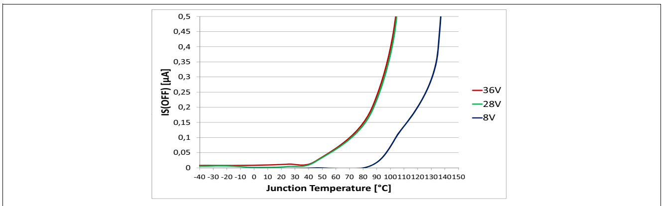
Figure 33 Standby Current for Whole Device with Load. I_{\text{S(OFF)}} = f(T_J; V_S)
