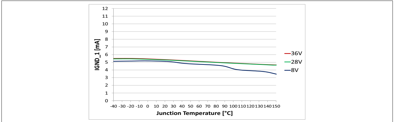
Figure 31 Current Consumption for Whole Device with Load. One Channel Active I_{\text{GND}_1} = f(T_J; V_S)
