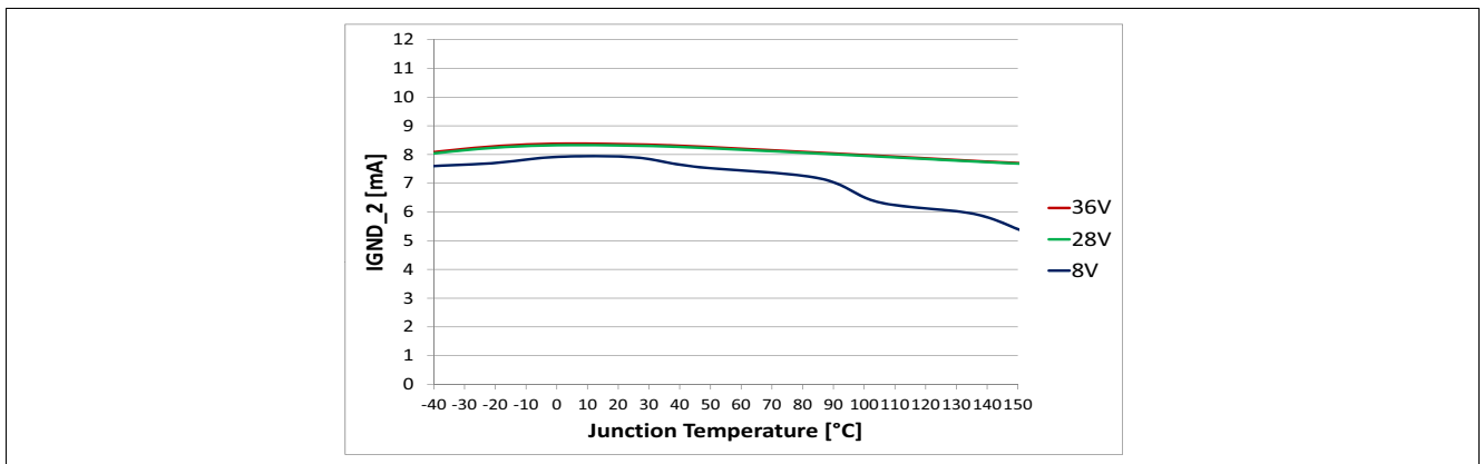
Figure 32 Current Consumption for Whole Device with Load. Two Channels Active I_{\text{GND}_2} = f(T_J; V_S)
