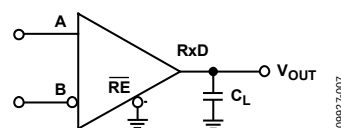
Figure 33. Receiver Propagation Delay
