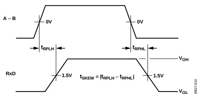
Figure 36. Receiver Propagation Delay
