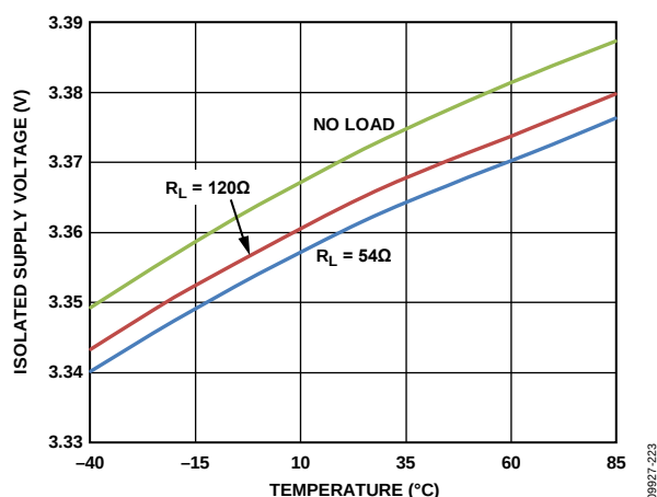
Figure 23. ADM2682E Isolated Supply Voltage vs. Temperature ( V_{CC} = 3.3 V, Data Rate = 16 Mbps)
