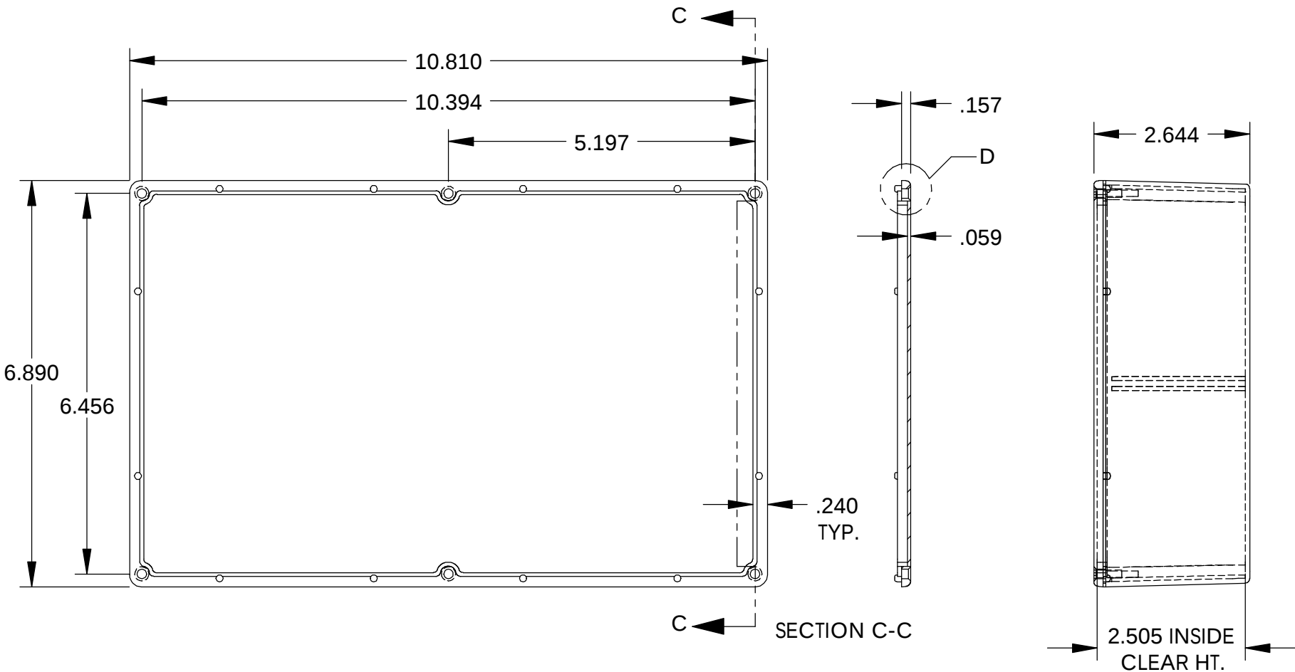
COVER
