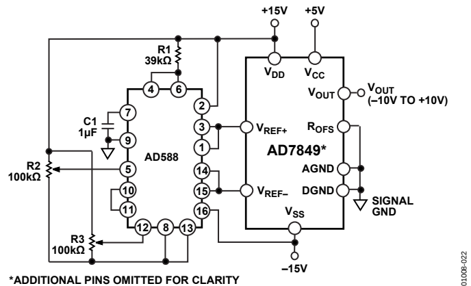
Figure 21. Bipolar \pm 10 \text{ V} Operation
