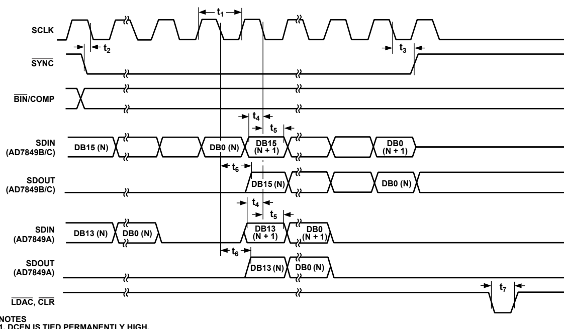
Figure 18. Timing Diagram (Daisy-Chain Mode)
