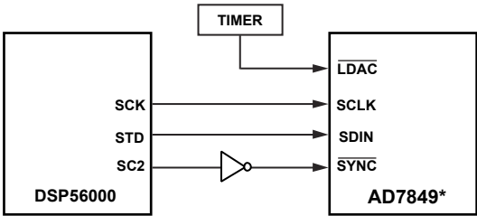
Figure 24. AD7849-to-DSP56000 Interface
