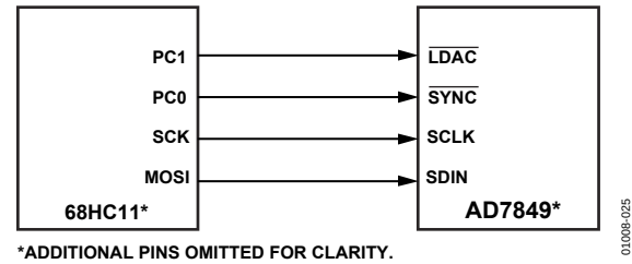
Figure 26. AD7849-to-68HC11 Interface
