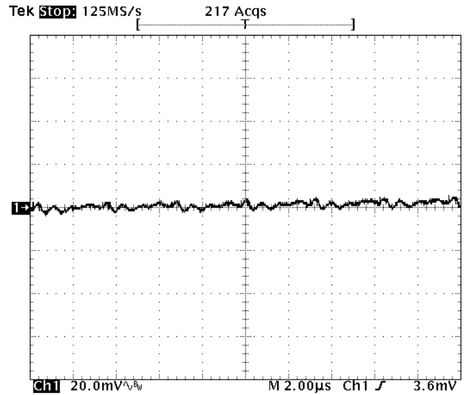
Fig-1.0V-5: Output voltage ripple (20mV/div.) for V_{out}=1.0V at full rated load current into a resistive load with external capacitance 47\mu F \times 4 ceramic + 1uF ceramic at V_{in}=12V . Time scale: 2 us/div
