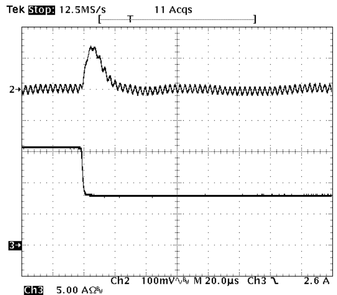
Fig-3.3V-7: Output voltage response for V_{out}=3.3V to negative load current step change from 16A to 8A with slew rate of -5A/us at V_{in}=12V . C_o=47\mu F \times 4 ceramic. Top trace: output voltage (100mV/div.) Bottom trace: load current (5A/div.) Time scale: 20us/div.
