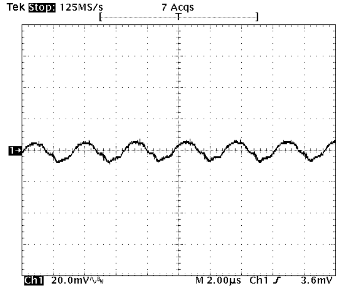
Fig-3.3V-5: Output voltage ripple (20mV/div.) for V_{out}=3.3V at full rated load current into a resistive load with external capacitance 47\mu F \times 4 ceramic + 1\mu F ceramic at V_{in}=12V . Time scale: 2 us/div
