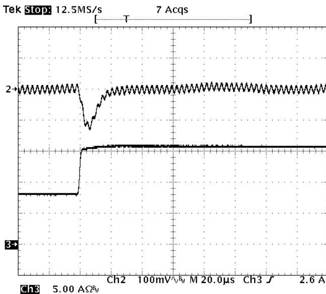
Fig-3.3V-6: Output voltage response for V_{out}=3.3V to positive load current step-change from 8A to 16A with slew rate of 5A/us at V_{in}=12V . C_o=47\mu F \times 4 ceramic. Top trace: output voltage (100mV/div.) Bottom trace: load current (5A/div.) Time scale: 20us/div.
