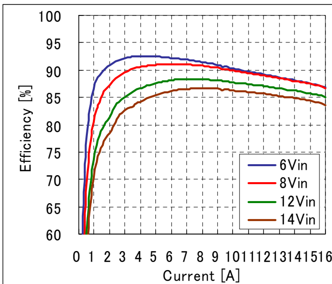
Fig-1.2V-2: Efficiency vs. load current and input voltage for Vout=1.2V. Airflow rate=200 LFM (1m/s) and Ta=25°C.
