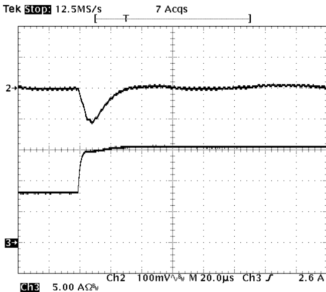
Fig-1.0V-6: Output voltage response for V_{out}=1.0V to positive load current step change from 8A to 16A with slew rate of 5A/us at V_{in}=12V . C_o=47\mu F \times 4 ceramic. Top trace: output voltage (100mV/div.) Bottom trace: load current (5A/div.) Time scale: 20us/div.
