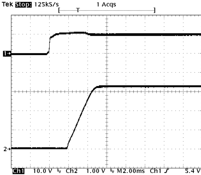
Fig-3.3V-4: Turn-on transient for V_{out}=3.3V with application of V_{in} at full rated load current (resistive) and 47\mu F \times 4 external capacitance at V_{in}=12V . Top trace: V_{in} (10V/div.) Bottom trace: output voltage (1V/div.) Time scale: 2ms/div.
