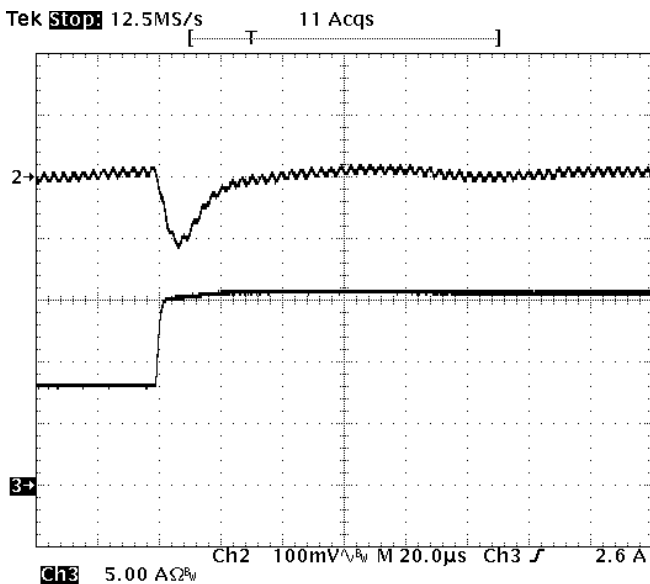
Fig-2.0V-6: Output voltage response for V_{out}=2.0V to positive load current step change from 8A to 16A with slew rate of 5A/us at V_{in}=12V . C_o=47\mu F \times 4 ceramic. Top trace: output voltage (100mV/div.) Bottom trace: load current (5A/div.) Time scale: 20us/div.
