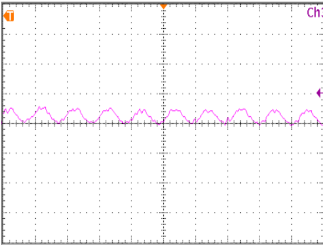
Figure 12: Input reflected ripple current, i_s , through a 12\mu\text{H} source inductor at nominal input voltage and max load current ( 25\text{mA}/\text{div} \cdot 4\mu\text{s}/\text{div} ).
